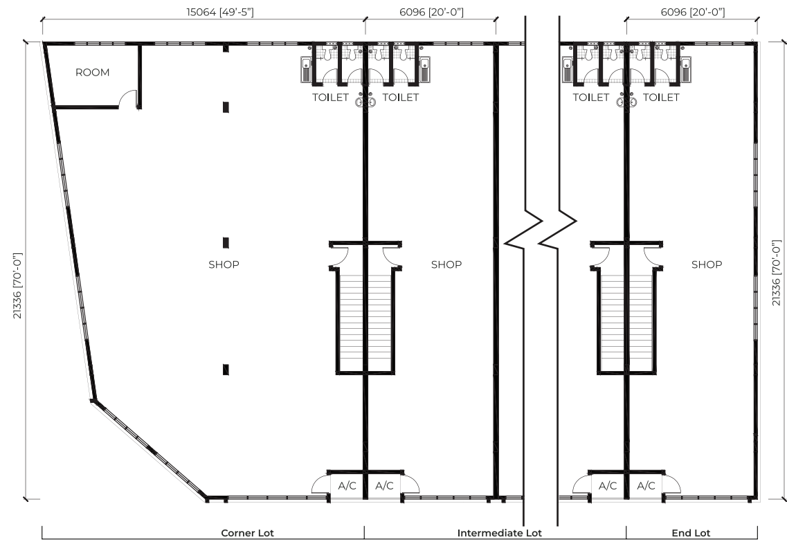
1ST FLOOR
